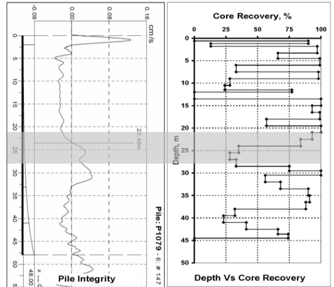
Figure 11. Comparison of PIT with concrete core recovery
