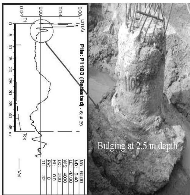
Figure 6. PIT results confirmed by excavation (Pile No. 1103)
